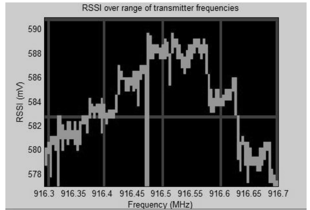
Figure 1: RSSI for one node from 916.3 to 916.7MHz
