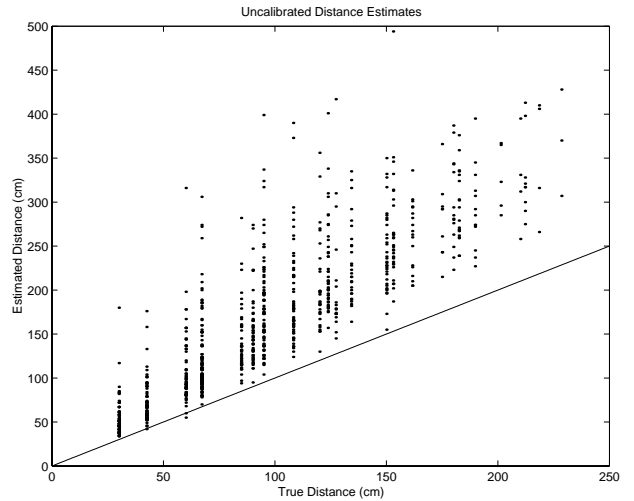
Figure 4: Uncalibrated TOF readings
